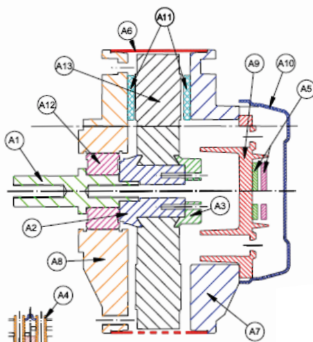
SECTION A-A Scale 0.75
